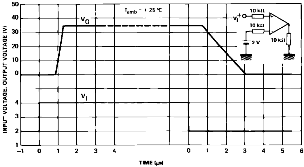
Figure 13 : Response Time.
